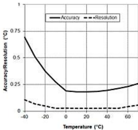
Plot A: Internal Temperature Accuracy & Resolution
